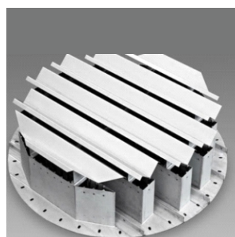
Liquid Collector/ Liquid Distributor
