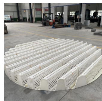
Packing Support/ Grid Support
